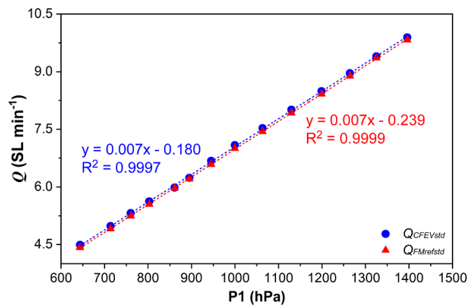
Figure 12. The gas flow past PT A as measured by the Gilibrator calibrated FM ( Q_{FMrfstd} ) and the gas flow as measured by the CFEV method ( Q_{CFEVstd} ) as the pressure to the inlet of the choked flow restriction ( P_{up} ) is varied away from 1 atm.
