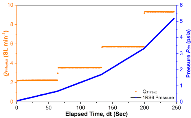
Figure 9. This plot shows the flow rate Q_{FMrfstd} (red) and the pressure P_{dn} (blue) vs elapsed time dt for an experiment wherein four different flow rates for a single evacuation/refilling of the vessel were achieved. Compressed air was used and the needle valve was in FWD orientation.
