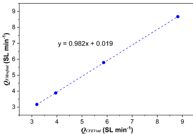
Figure 10. Q_{FMrfstd} vs Q_{CFEVstd} for four different flow rates for one vessel evacuation/refilling. The valve used was the Swagelok MN SS-1RS6.
