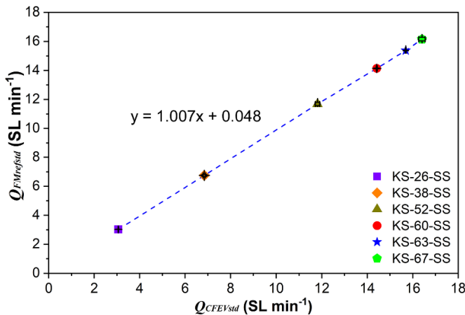
Figure 6. The measured flow rate Q_{\text{FMrefstd}} vs the computed flow rate Q_{\text{CFEVstd}} for six different orifices. For each data point, there were three trials. The vertical error bars were taken from the standard deviations of the average readings and they are too small to be seen.
