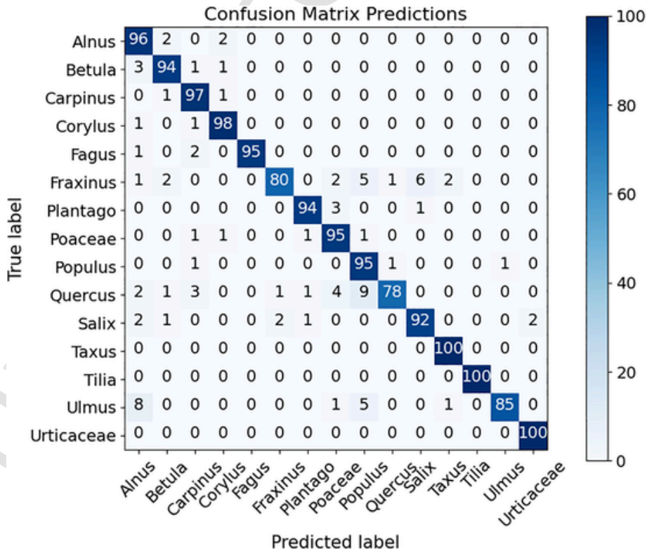
Fig. 3. Normalised confusion matrix for our best Dataset-15 configuration, averaged over five runs. Results are rounded to integer percentage points.
