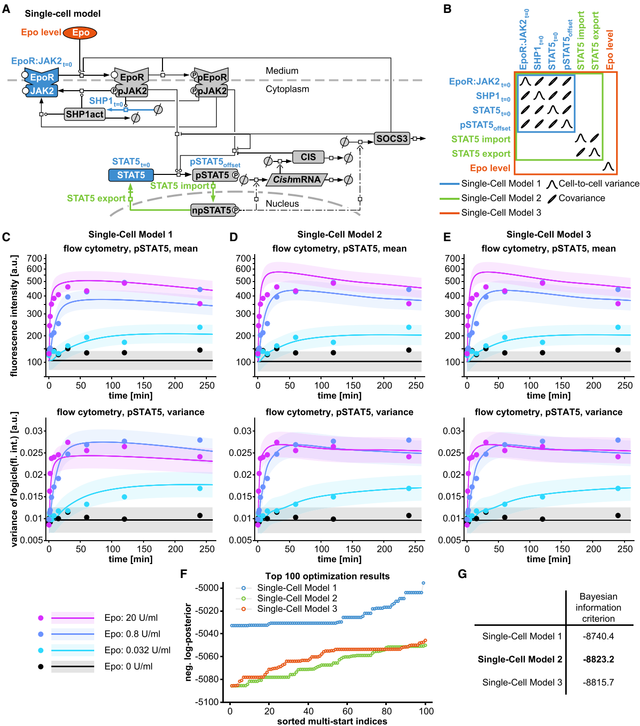
Figure 4. Dynamic mathematical JAK2/STAT5 pathway model describing cell-to-cell variability of phosphorylated STAT5 (A) The structure of the single-cell model of the JAK2/STAT5 pathway with putative sources of cell-to-cell variability of pSTAT5 (colored corresponding to the different models). (B) Visualization of covariance matrix for the three candidate models. (C–E) Experimental data (mean and variance of pSTAT5 from flow cytometry) and mixed-effect model outputs. See Figure S4 for correlation of data and model output and Figure S5 for full flow cytometry dataset and model output. (F) Multi-start optimization results for candidate single-cell models. Best 100 of 400 local optimization runs are shown, and plateaus indicate convergence. (G) Bayesian information criterion (BIC) values of the three candidate models.
