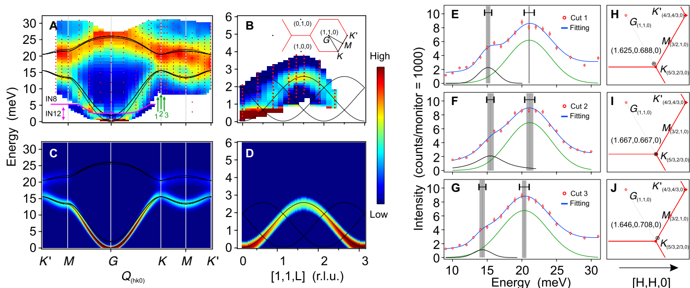
Fig. 3. Spin-wave excitations in CrGeTe 3 . (A and B) Energy- and momentum-resolved neutron scattering intensity maps of magnon in CrGeTe 3 along the high-symmetry directions measured at IN8 and IN12, respectively. Black solid lines are the calculated magnon dispersion curves. Inset in (B) shows the projected BZ with high-symmetry points and the scan paths in the experiments. (C and D) The corresponding calculated magnon spectra intensity maps for (A) and (B) by using the 2nd-NN DM interaction model. The calculated spectra are convolved with an energy resolution of 1 meV to compare with experimental data. (E to G) The line profiles of constant-Q energy scan at the positions of 1, 2, 3 marked by the green arrows in (A) near the K point Q=(5/3, 2/3, 0) . The solid lines are the multipeak Gauss fitting results. The peak positions and the errors are indicated, respectively, by the dashed lines and the gray shadows; the corresponding energy resolutions are represented by the black horizontal bar with caps. (H to J) The actual Q positions of the cut 1, 2, and 3 are marked by black circles with center dots in the reciprocal space. The red solid lines are the BZ boundaries.
