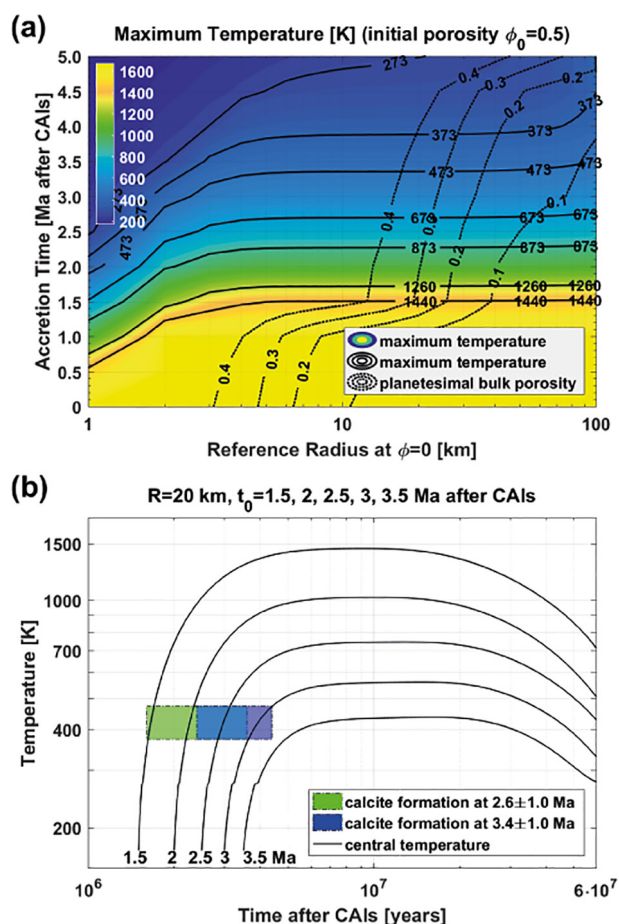
Fig. 27. (a) Maximum temperature and bulk porosity as functions of the accretion time and size of the parent body. A maximum temperature of 400^\circ\text{C} is obtained for planetesimals with an accretion time of \sim 2.7 Ma after CAIs. The thermal evolution of these bodies is consistent with the Mn-Cr data. Bulk porosities of 30%, 20%, and 10% are obtained for radii of \sim 20 km, \sim 30 km, and \sim 60 km, respectively. (b) Thermal evolution of the Flensburg parent body at the center assuming accretion at 1.5, 2, 2.5, 3, and 3.5 Ma after CAIs, and a radius of 20 km. Calcite formation of 2.6 Ma or 3.4 Ma after CAIs can be fitted on prograde temperature evolution paths. High maximum temperatures obtained assuming accretion at 1.5 and 2 Ma after CAIs imply phyllosilicate dehydration or partial melting, contradicting Flensburg mineralogy. Maximum temperatures of 350\text{--}400^\circ\text{C} ( 623\text{--}673 K) obtained in the Flensburg parent body assuming accretion at \sim 2.7 Ma after CAIs agree with mineralogical observations, and this accretion time is compatible with both calcite formation ages.
