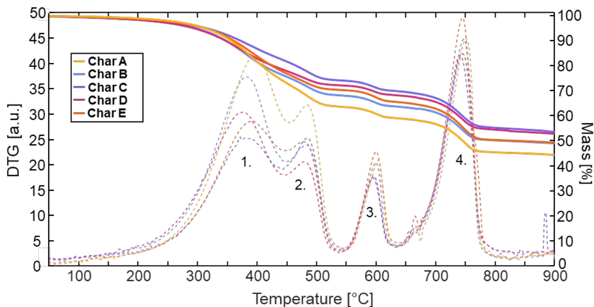
31 32 33 34 35 36 37 38 39 40 41 42 43 44 45 46 47 48 49 50 51 52 Figure 1. Mass loss (solid line) and differential thermogravimetric (DTG, dashed line) results of the 53 plastic waste pyrolysis char thermal investigation. Several distinct decomposition steps similar to all 54 five char samples but differently pronounced can be observed. Due to the similar nature of all pyrolysis 55 char samples, Char A was selected for all further visualization. 56 57 58
