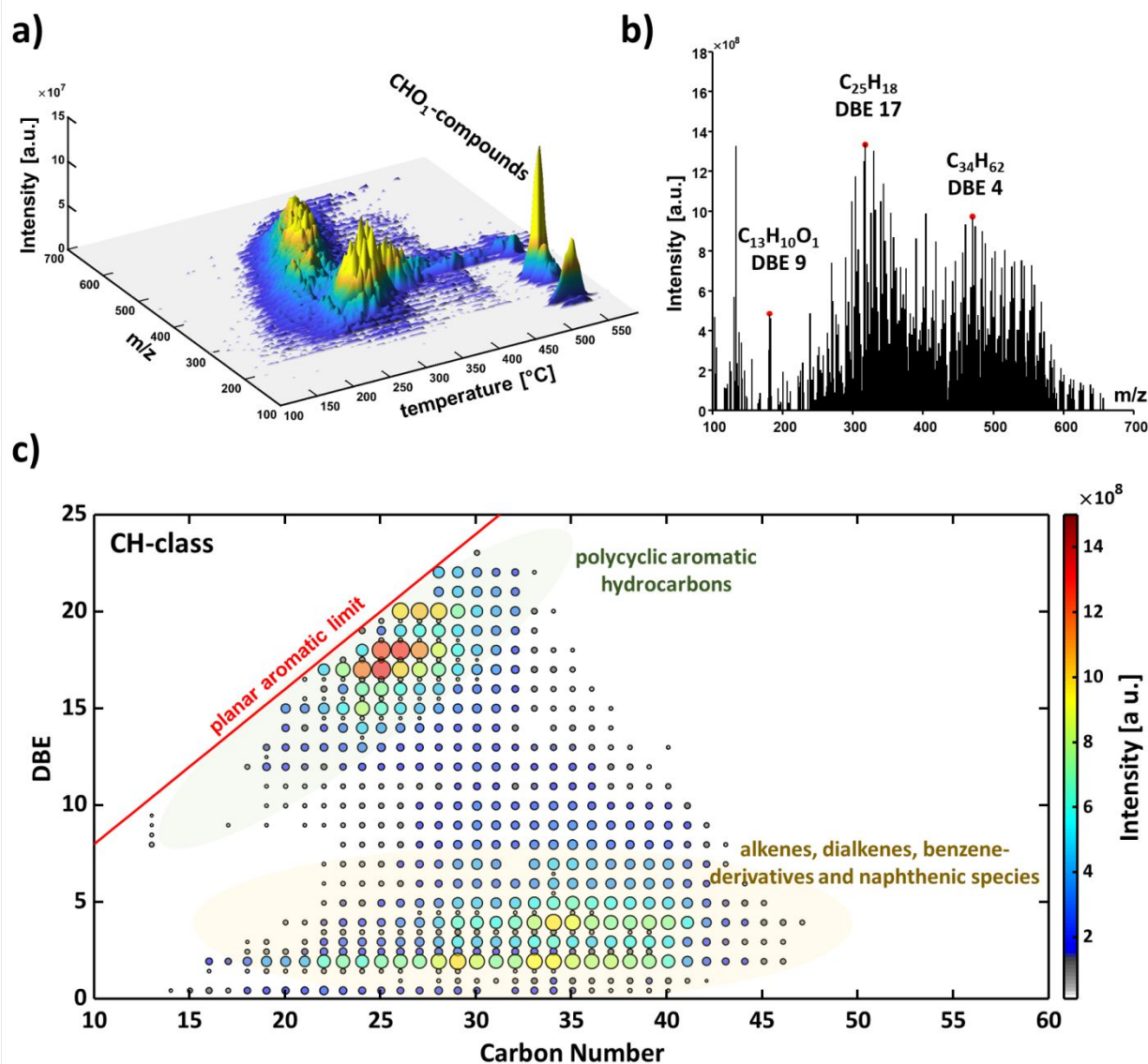
Figure 5. Compilation of the results from the thermal analysis ultrahigh-resolution mass spectrometric char analysis (TG FT-ICR MS) of Char A. a) Survey data visualization of the general mass spectrometric response (temperature versus m/z ). b) Average mass spectrum of the attributed elemental compositions. c) Double bond equivalent (DBE) versus carbon number (#C) diagram of the CH-class. Two distinct chemical distributions, one at higher DBE values with comparable low #C spread and second at low DBE 0-5 with a high #C spread, attributed to polycyclic aromatic hydrocarbons and alkenes, dienes, benzene-derivatives, and naphthenic species, can be found, respectively.
