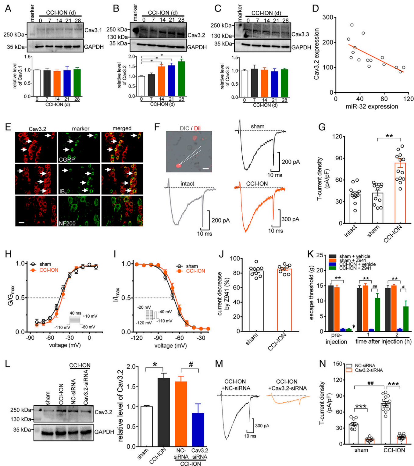
Fig. 6. Cav3.2 protein increases in TGs after CCI-ION. (A–C) Protein expression levels of Cav3.1 (A), Cav3.2 (B), and Cav3.3 (C) in rat TGs on days 0, 7, 14, 21, and 28 post-CCI-ION. * P < 0.05 (vs. control [0 d], one-way ANOVA). Depicted immunoblots are representative of three independent experiments. (D) Linear regression analysis showed that the miR-32-5p level was inversely related to the Cav3.2 expression level in the ipsilateral TGs ( R^2 = 0.4805 ). (E) Representative images of double immunostaining of Cav3.2 with CGRP, IB _4 , and NF200 in rat TG sections. White arrows indicate double-labeled neurons. (Scale bar, 50 \mu m.) (F) Representative current traces of T-type channel currents recorded from retrograde Dil-labeled small TG neurons on day 14 post-CCI-ION or after sham operation. (F, inset) Recording from a Dil-labeled TG neuron. (Scale bar, 50 \mu m.) (G) Summary of results showing the T-type channel current density in small TG neurons on day 14 post-CCI-ION or after sham operation ( n = 12 to 15 neurons per group). No significant changes were observed between the intact and sham-operated groups. ** P < 0.01 (vs. sham, one-way ANOVA). (H and I) Nerve injury induced by CCI-ION (14 d) did not affect voltage-dependent activation ( n = 12 neurons per group; H ) or the steady-state inactivation profile ( n = 15 neurons per group; I ) of T-type channels. H and I , Insets indicate stimulation protocols. (J) Application of Z941 at 0.5 \mu M dramatically decreased T-type channel currents in TG neurons on day 14 post-CCI-ION ( n = 9 neurons per group) or after sham operation ( n = 8 neurons per group). (K) Intra-TG injection of Z941 (2 nmol) alleviated mechanical allodynia on day 14 post-CCI-ION. ** P < 0.01 (vs. vehicle + sham); # P < 0.05 ; ### P < 0.01 (vs. CCI-ION + vehicle) (two-way ANOVA). (L) Intra-TG injection of Cav3.2 siRNA (Cav3.2-siRNA) attenuated the increased protein expression of Cav3.2 in the ipsilateral TGs on day 14 post-CCI-ION. n = 7 or 8 rats per group. * P < 0.05 (vs. sham); # P < 0.05 (vs. CCI-ION + NC-siRNA) (one-way ANOVA). The immunoblots shown are representative of three independent experiments. (M) Representative current traces of T-type channel currents recorded from retrograde Dil-labeled small TG neurons on day 14 post-CCI-ION. (N) Summary of results showing the T-type channel current density in small TG neurons on day 14 post-CCI-ION or after sham operation ( n = 10 to 16 neurons per group). *** P < 0.001 (vs. NC-siRNA); ## P < 0.01 (vs. NC-siRNA + sham) (one-way ANOVA).
