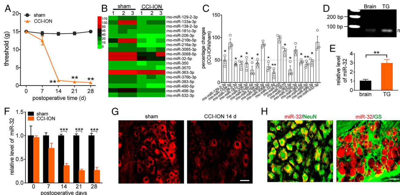
Fig. 1. miR-32-5p is down-regulated in TG neurons after CCI-ION. (A) Orofacial response threshold (threshold) to mechanical stimuli in the sham-operated and CCI-ION-operated groups ( n = 10 rats per group). ^{**}P < 0.01 (vs. sham, two-way ANOVA). (B) Heat map indicating TG-rich miRNAs showing significant expression decrease in injured TGs. (C) qPCR analysis indicating that 12 miRNAs are down-regulated by >50% in ipsilateral TG tissue on day 14 post-CCI-ION. ^{*}P < 0.05 ; ^{**}P < 0.01 (in CCI-ION vs. sham, unpaired t test). (D) RT-PCR analysis of miR-32-5p (miR-32) in the brains and TGs of intact rats. The blots shown are representative of three independent experiments. (E) qPCR of miR-32-5p expression in rat brain and TGs ( n = 5 rats per group). ^{**}P < 0.01 (vs. brain, unpaired t test). (F) The time course of miR-32-5p expression in the ipsilateral TGs in sham and CCI-ION-operated rats ( n = 5 to 7 rats per group). ^{***}P < 0.001 (vs. sham, one-way ANOVA). (G) Representative images of miR-32-5p expression in ipsilateral TG tissue on day 14 after CCI-ION or sham operation. (Scale bar, 50 \mu\text{m} .) (H) In situ hybridization of miR-32-5p and immunostaining with NeuN or GS. (Scale bar, 50 \mu\text{m} .)
