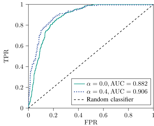
FIGURE 11. ROC curve. Opposing TPR and FPR in case of undersized mask ( \gamma = 0.1 ) comparing a random classifier to the proposed annotation inspection intra-annotator inspection considering ( \alpha = 0.4 ) and not considering ( \alpha = 0.0 ) uncertainty.
