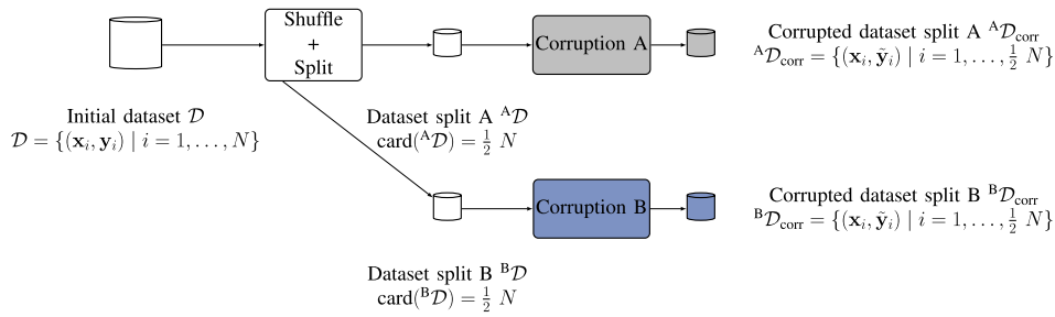
FIGURE 4. Inter-annotator variability simulation with two independent annotators. A clean dataset \mathcal{D} is split in two equal-sized parts to insert corruptions A,B to generate noisy datasets ^A \mathcal{D}_{\text{corr}}, ^B \mathcal{D}_{\text{corr}} .
