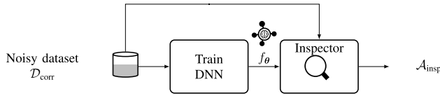
FIGURE 5. Inspection pipeline intra-annotator variability. The noisy dataset \mathcal{D}_{\text{corr}} is used to obtain an uncertainty-aware DNN f_\theta . The inspector uses the DNN to automatically predict an ordered list \mathcal{A}_{\text{insp}} which can be used for re-inspection of potentially noisy annotations.
