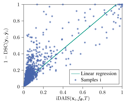
FIGURE 9. Evaluation of uncertainty estimation. Comparison of prediction error 1 - DSC(y_i, \tilde{y}_i) to iDAIS(x_i, f_\theta, T) of clean training dataset samples i and linear line fit.
