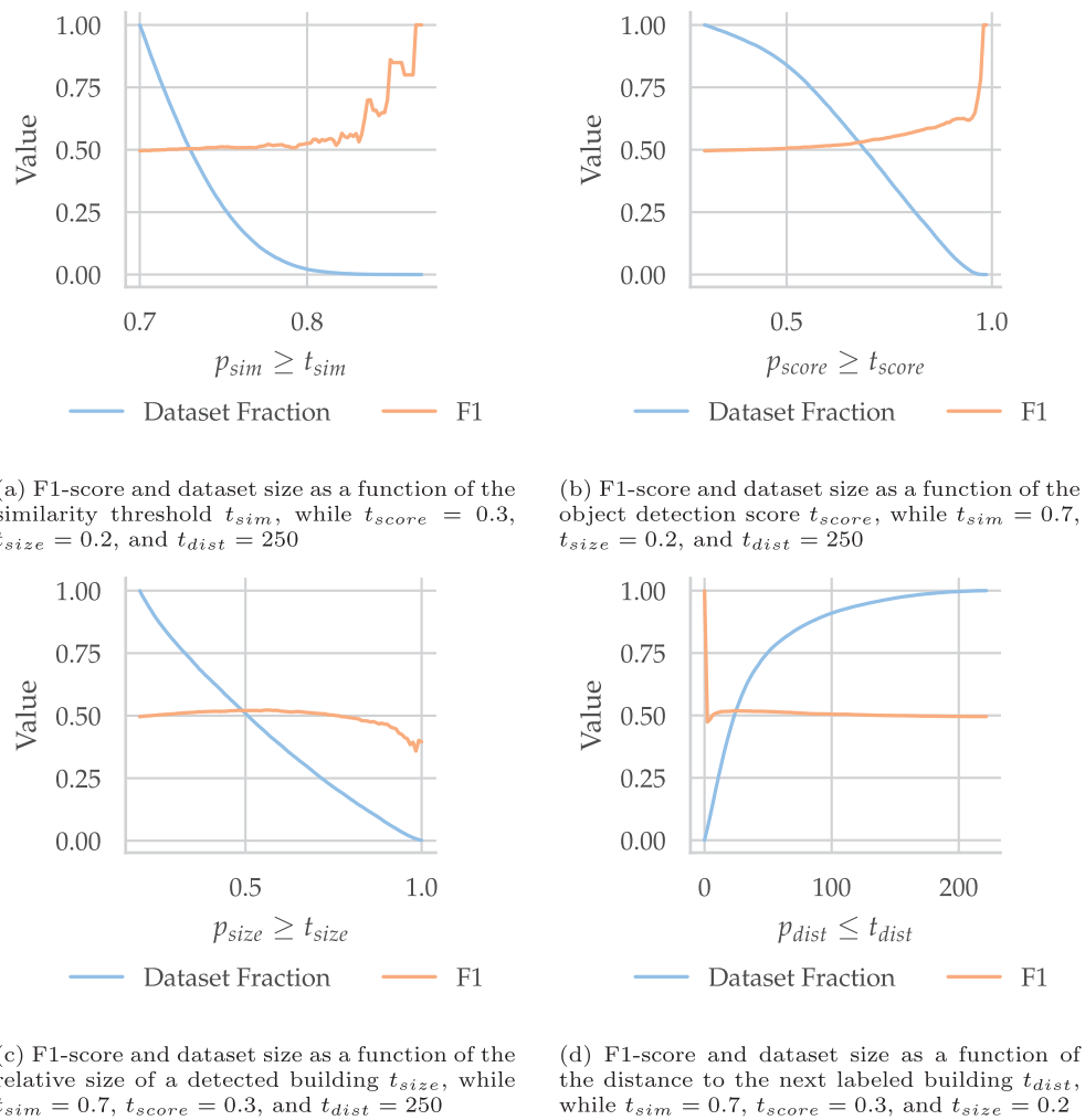
Fig. 2. Effect of filtering pipeline parameters on prediction results and remaining dataset size.
