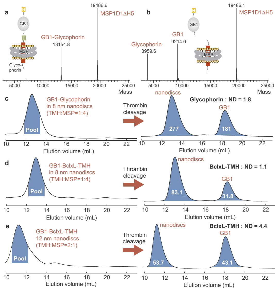
Fig. 4. Analysis of the oligomeric state of transmembrane helices by the GB1 assay. (a,b) Mass spectrometry (MS) analysis of nanodiscs containing the dimeric transmembrane helical protein glycoporinA (GlyA). After nanodisc assembly (a) as well as after Thrombin cleavage (b), the correct mass of the MSP and the inserted GlyA-GB1-fusion protein, GB1 and free GlyA could be detected. (c) Determination of the insertion number of GlyA in nanodiscs yields a value of 1.8 at an assembly ratio of 1:4 (GlyA:MSP). (d) As a comparison, the assay reports a value of 1.1 for the transmembrane helix of the anti-apoptotic protein BclxL in small nanodiscs if a low TMH-to-MSP ratio is used during assembly. (e) A value of 4.4 is obtained in larger 12 nm nanodiscs (assembled with MSP1E3D1) and if using a TMH-to-MSP ratio of 2:1 (leading to an expected number of 4 TMHs per nanodisc). In the BclxL-TMH case, TMH insertion is governed by the assembly conditions suggesting that no dimerization but rather co-assembly takes place.
