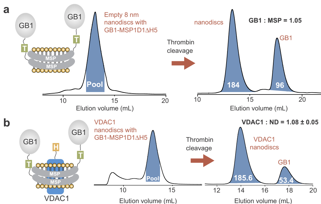
Fig. 5. Fusion of GB1 to MSP yields proper nanodisc assembly and correct insertion numbers. (a) The use of GB1-MSP1D1ΔH5 yields properly assembled nanodiscs (left panel) that can be cleaved with thrombin for the determination of the molar ratio of GB1 and MSP (right). In case of GB1-MSP fusion proteins, this ratio must be 1. Thus, such samples can be used to adjust the calculated molar extinction coefficient ( \epsilon_{280} ) of GB1 by the offset from the expected 1:1 ratio. (correction by 5%, resulting in an \epsilon_{280} of 10,006 \text{ M}^{-1} \text{ cm}^{-1} instead of the calculated value of 9530 \text{ M}^{-1} \text{ cm}^{-1} ). This value was used for all calculations in this study. In this setup, GB1 reports on the amount of MSP. (b) Using VDAC1-loaded nanodiscs, a calculation similar to Eqs. (1)–(3) can be utilized to derive the VDAC1:nanodisc ratio, which is shown for VDAC1 in GB1-MSP1D1ΔH5 nanodiscs to be 1.08 \pm 0.05 (average and standard deviation derived from 3 independent experiments). T: thrombin cleavage site; H: His 6 -tag.
