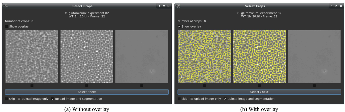
Fig 3. Crop creation interface. Automatically proposed crops can be selected and uploaded to OMERO (a). The crop proposals are extracted randomly from different non-overlapping image regions (the left crop originates from the left image region, and the right crop from the right). For the pre-labeling, it is possible to upload only the image or the image with its prediction (b). The image-only upload is helpful when the pre-label predictions require too many manual corrections.
