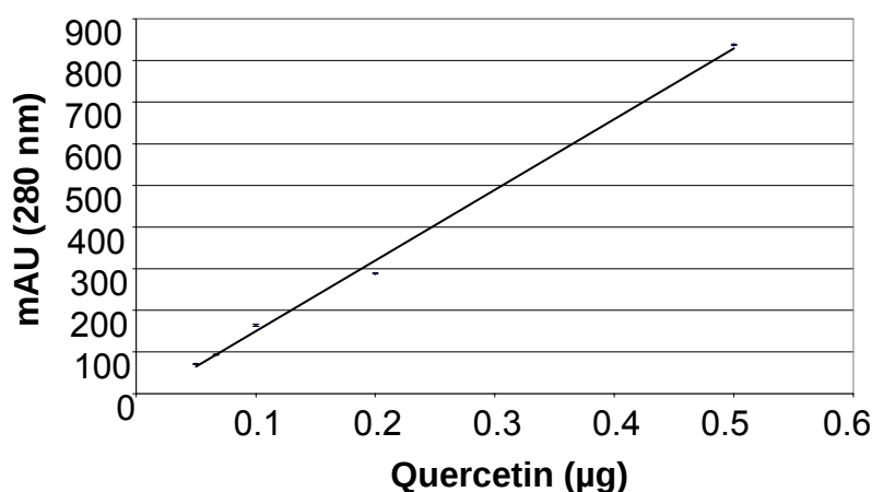
Figure 2. 4 The quercetin calibration curve. The formula of the calibration curve obtained is y = 1700x - 20.607 ( y = \text{mAU} , x = \mu\text{g} ). The error bars are means \pm SD, n = 3 . The error bars are very small.
