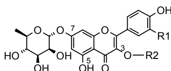
Figure 1. 3 Major flavonol glycosides in Arabidopsis (accession Columbia). R1 = H (kaempferol), = OH (quercetin). R2 = glucose (flavonol-3-O-glucoside-7-O-rhamnoside), = rhamnose (flavonol-3-O-rhamnoside-7-O-rhamnoside), or = rhamnose (1->2)-glucose (flavonol-3-O-[rhamnosyl (1->2) glucoside]-7-O-rhamnoside).
