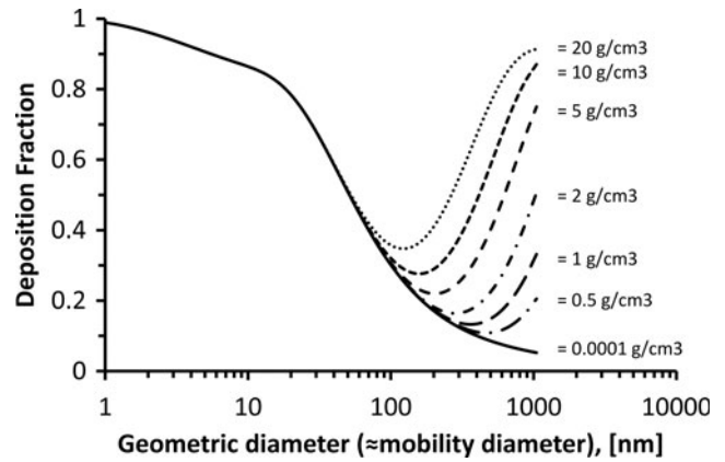
FIG. 2. Size-resolved total DF as a function of particle density ( 0.0001 – 20 \text{ g}/\text{cm}^3 ). Data are calculated with the ICRP model for a sitting male adult (nose breathing; tidal volume, 0.75 \text{ L} ; breathing frequency, 12 \text{ min}^{-1} ). (5) For small enough particles, DF is independent of particle density (diffusion-dominated regime). The upper limit of the diffusion-dominated regime is between 100 and 600 nm for densities between 20 and 0.5 \text{ g}/\text{cm}^3 . For a density of 1 – 2 \text{ g}/\text{cm}^3 (typical for ambient particles), the upper size limit of the diffusion-dominated regime is about 300 nm, because at this size DF is twice the value of the zero density line (here: 0.0001 \text{ g}/\text{cm}^3 ), which represents DF due to diffusion only.
