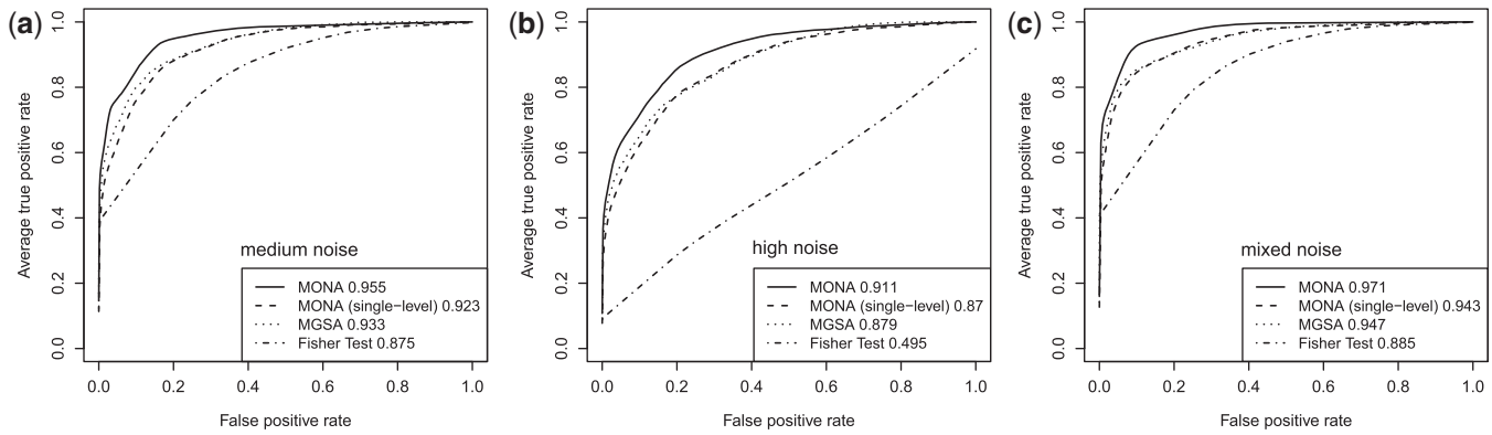
Figure 3. Performance of the cooperative model on synthetic data for three different levels of noise: (a) medium noise ( \alpha^{I/II} = 0.25 , \beta^{I/II} = 0.25 ), (b) high noise ( \alpha^{I/II} = 0.25 , \beta^{I/II} = 0.4 ) and (c) mixed noise ( \alpha^{I/II} = 0.1 , \beta^{I/II} = 0.4 ). AUC values are listed in the respective figure legends. With MONA, the inference is based on two species, and all other algorithms are based on one species only.
