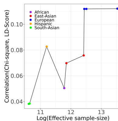
FIGURE 1 | Effective sample size against the correlation between \chi^2 -values and LD scores from ancestry-specific meta-analyses part of DIAMANTE-18, DIAMANTE-22 and T2DGGI-24 meta-analyses.
