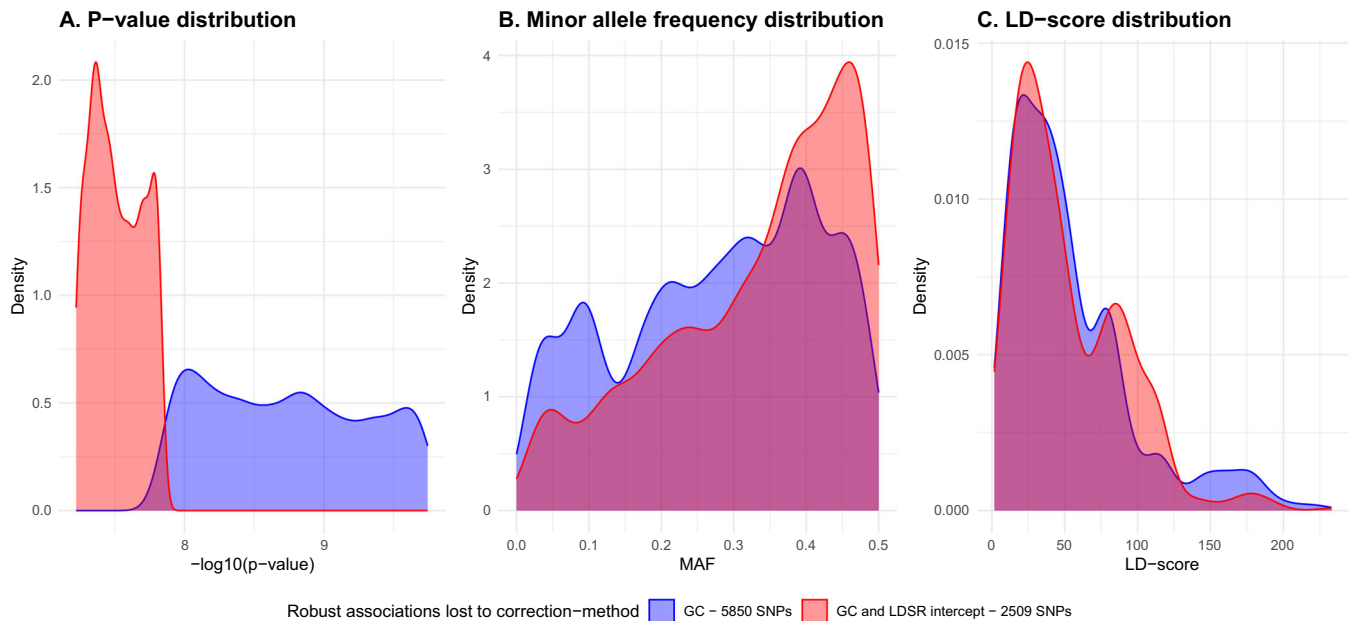
FIGURE 3 | Distributions of p values, MAF and LD-scores for robust associations lost only to GC correction compared to those lost to both GC and LDSR intercept correction in the DIAMANTE-18 and the DIAMANTE-22 analysis. p value distribution: t -test p < 2 \times 10^{-16} . Minor allele frequency distribution: t -test p < 2 \times 10^{-16} . LD score distribution: t -test p = 0.346 . (A) P -value distribution (B) Minor allele frequency distribution (C) LD-score distribution 0.015
