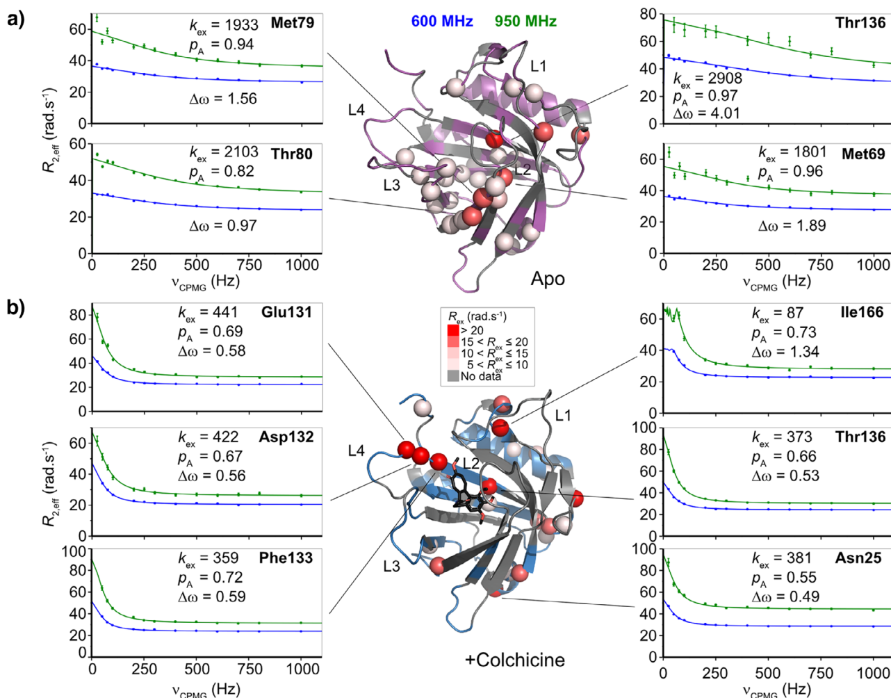
Figure 2. Microsecond-to-millisecond timescale backbone dynamics for Colchicalin in the apo and colchicine-bound states. 15 N CPMG relaxation dispersion profiles recorded at 600 MHz (blue) and 950 MHz (green) ( 1 H frequency) are shown for the a) apo and b) colchicine-bound states. R_{ex} contributions at 950 MHz > 5 rad.s -1 are plotted on the corresponding X-ray structures as spheres and dispersion profiles for selected residues are shown. Fitted values for k_{ex} (rad.s -1 ), p_A (%) and \Delta\omega (ppm) are indicated on the graphs. Fitted values for all residues are shown in Figure S4.
