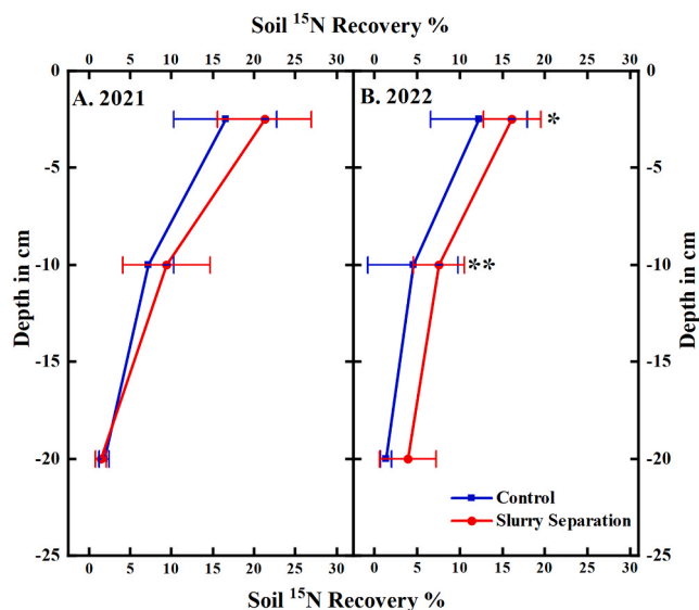
Fig. 4. Soil 15 N recovery at different depths (0–5 cm; 5–15 cm; 15–25 cm) based on the cumulative 15 N excess addition at the time of sampling. Fig. A represents soil 15 N recovery after the first experimental year, sampled in March 2022; and B represents soil 15 N recovery after two years, sampled in March 2023. Asterisks represent significant differences between control and separate slurry treatments at the same depth ( p < 0.05 ).
