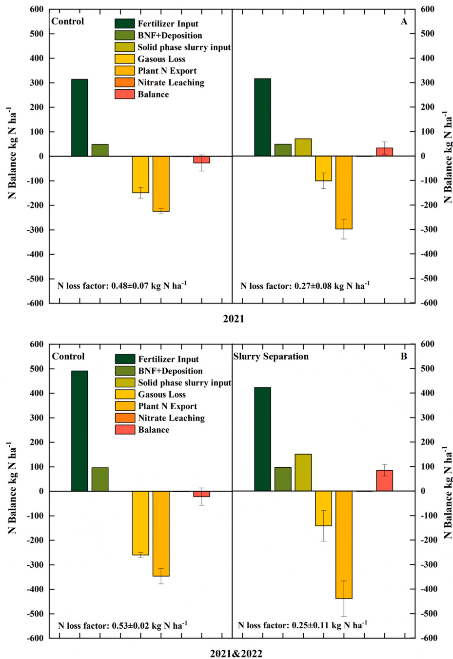
Fig. 8. Total N balances for the control and slurry separation treatments in 2021 (A. 1-year balance) and 2022 (B. 2-year balance). The 2021 N balance was calculated at the end of the first experimental year, while the 2022 N balance was determined after the conclusion of both the first plus second experimental years. The N balance includes inputs from fertilizer, biological N fixation (BNF), and deposition, as well as gaseous losses and plant N export (including AGB and BGB). For these considerations, the SPS N inputs were considered to be stable, i.e., not undergo N loss. N loss factor: Average gaseous and leaching N losses per kg of added fertilizer N.
