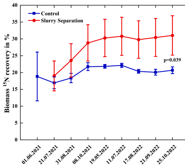
Fig. 3. Fertilizer ^{15}\text{N} recovery in aboveground biomass (% of added ^{15}\text{N} excess). ^{15}\text{N} recovery for the single sampling points is calculated by dividing the cumulative ^{15}\text{N} excess amount harvested at the given sample date by the amount of cumulative ^{15}\text{N} excess added with fertilizer until the respective sampling. Note that no ^{15}\text{N} was added during the addition of SPS, i.e., for the first harvest in 2021 and 2022 each.
