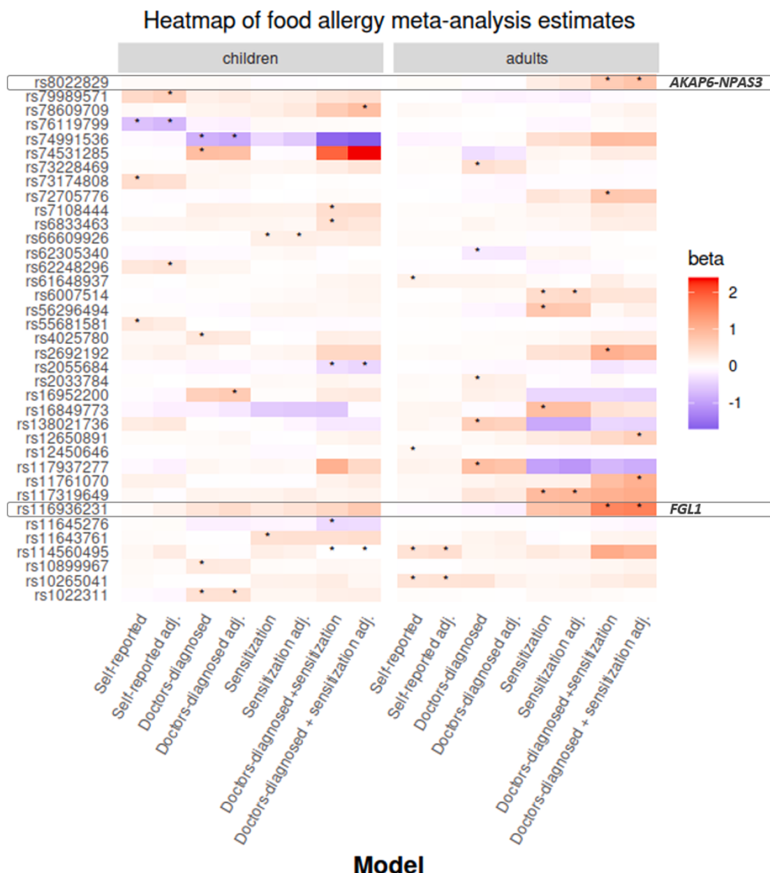
FIG 2. Heat map of effect estimates from GWAS meta-analyses by phenotype and age group for 37 lead SNPs. Lead SNPs are indicated on y-axis, and results per phenotype and model are displayed on x-axis. Asterisks indicate trait where significance threshold ( P < 1 \times 10^{-6} ) was passed in discovery. Genome-wide significant SNPs are outlined with box including mapped gene.
