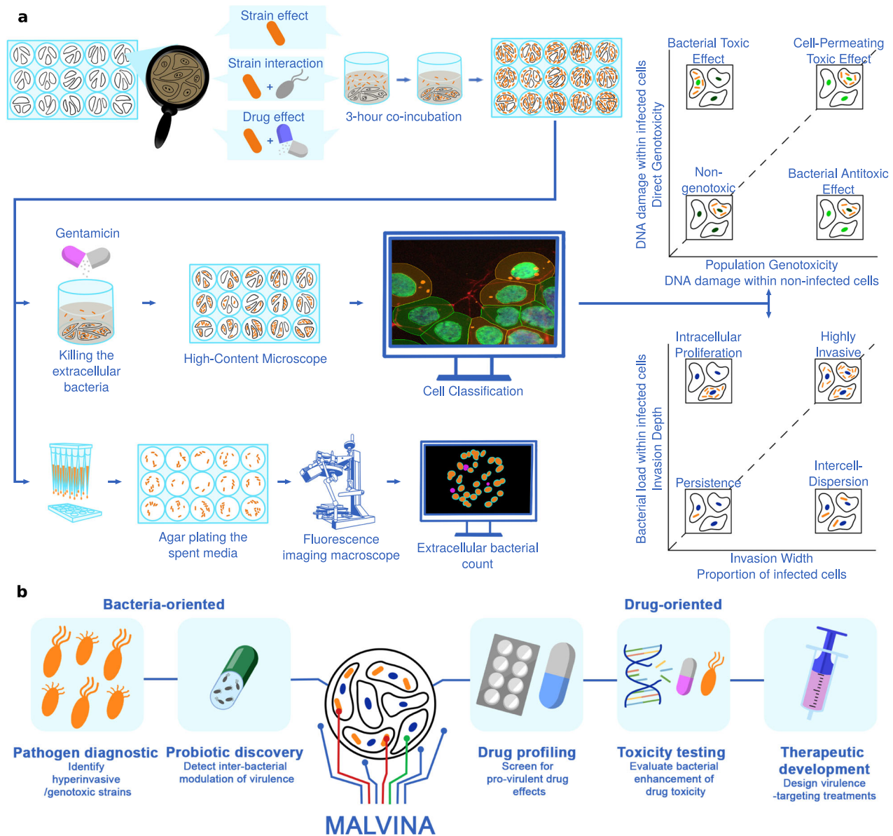
Fig. 1 | Schematic of the MALVINA workflow. a Human colorectal epithelial cells are seeded into 96-well plates, allowed to form monolayers, and infected for 3 h under one of three conditions: (i) a single fluorescently labelled strain, (ii) co-infection with labelled and unlabelled strains, or (iii) a labelled strain exposed to various drugs. After incubation, the workflow splits into two branches. Bottom branch: supernatant is collected, diluted, plated, and colonies counted to quantify extracellular bacteria—key for the drug screen. Top branch: monolayers are treated
