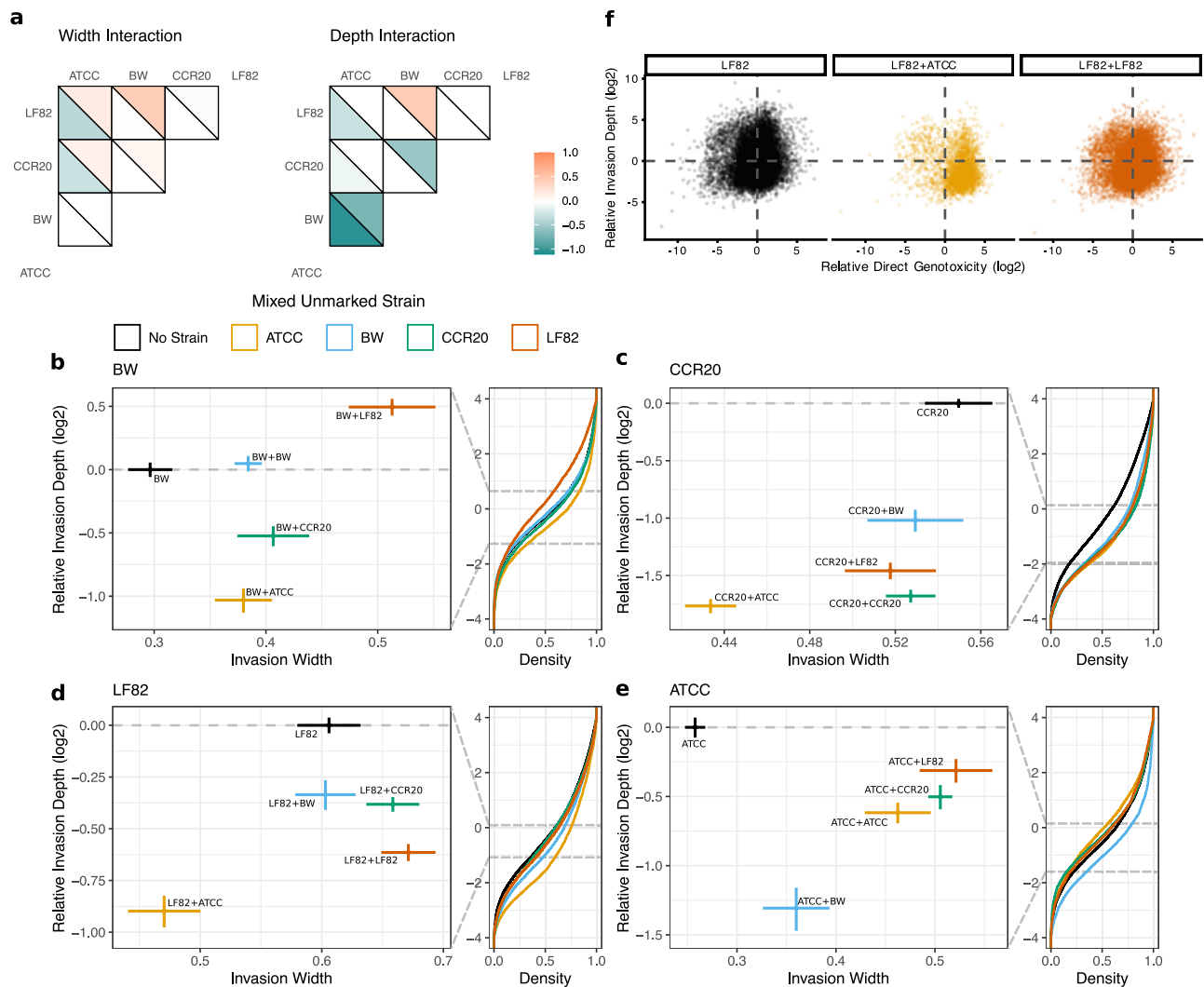
Fig. 3 | Mapping inter-strain modulation of bacterial invasion. a Directional interaction scores for the two key invasion traits, invasion width and invasion depth, across all pairwise combinations of the four E. coli strains. The top (bottom) triangles show the interaction score for the effect of the bacteria in the row (column) on the bacteria in the column (row). Orange indicates enhancement, cyan indicates suppression. b–e Invasion modulation landscapes for fluorescently labelled BW ( b ), CCR20 ( c ), LF82 ( d ), and ATCC ( e ) in the presence of the various unlabelled partner strains. Invasion depth is calculated relative to the corresponding fluorescently labelled single-strain control, indicated by the black cross in each plot. Geometrically normalised cumulative density plots show single-cell
