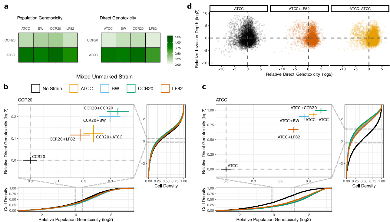
Fig. 4 | Inter-strain interactions enhance the genotoxic potency of colibactin-producing E. coli strains. Genotoxicity modulation matrix: unlabelled strains (columns) were co-cultured with the two labelled genotoxic strains (rows), and changes in direct and population-level genotoxicity are shown relative to the effect of the corresponding labelled single-strain reference. b, c Genotoxicity modulation landscapes for CCR20 ( b ) and ATCC ( c ) in the presence of various unlabelled strains. Each plot shows changes in population genotoxicity versus direct genotoxicity relative to the labelled single-strain reference, indicated by the black cross in each plot. Geometrically normalised cumulative density plots show single-cell
