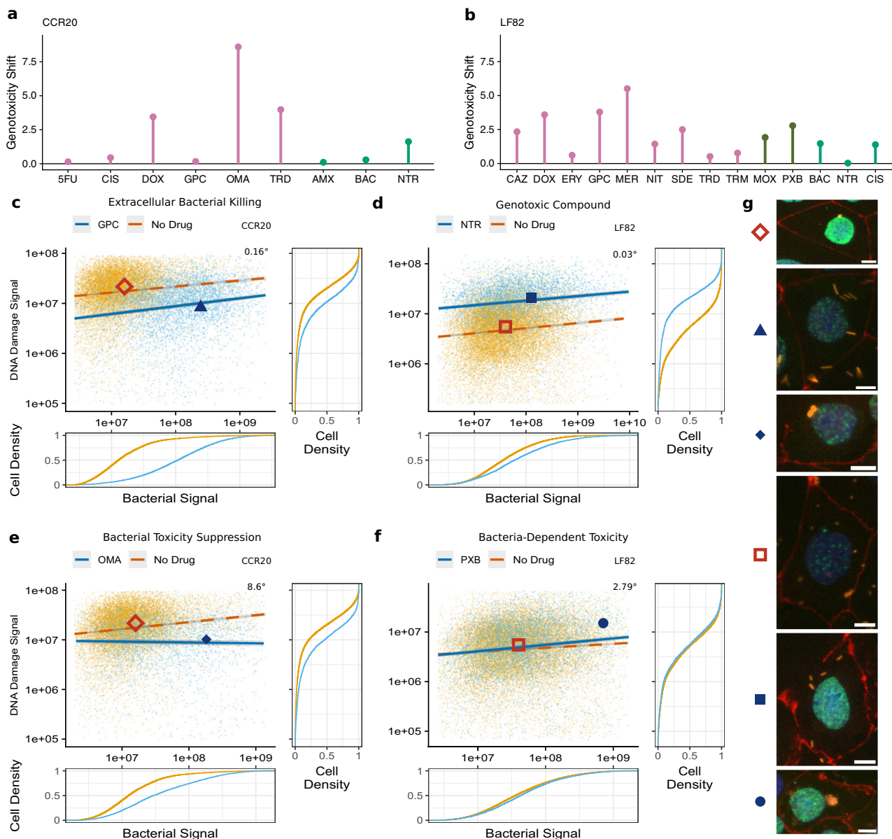
Fig. 7 | Genotoxicity shift reveals direct drug effects on bacteria-mediated genotoxicity. a, b Genotoxicity shifts for drugs from different genotoxicity-modulation classes during LF82 (a) or CCR20 (b) infection (see Fig. 6). The shift is defined as the absolute change in the slope angle of the log-log relationship between intracellular bacterial load and DNA damage in infected host cells, measured between drug-treated and untreated conditions (“Methods”). Bars are colour-coded by genotoxicity-modulation drug class (see legend of Fig. 6e, f). c–f Exemplars of genotoxicity shifts. Non-shifting drugs leave bacterial load-dependent genotoxicity unchanged (c N-nitroso-N-ethylurea, NTR; d gepotidacin, GPC), whereas shifting drugs alter the intracellular bacteria-dependent dynamics of genotoxicity (e polymyxin B, PXB; f omadacycline, OMA). Examples are shown for
