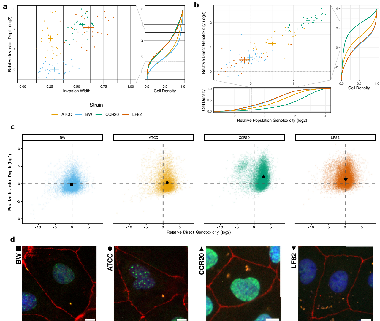
Fig. 2 | Single-cell quantification of bacterial invasion and genotoxicity reveals strain-specific virulence profiles. a, b Invasion (a) and genotoxicity (b) profiles of four E. coli strains. Invasion depth was calculated relative to the BW strain, while direct and population genotoxicity relative to uninfected controls. Each point is a replicate measurement; crosses show the mean \pm confidence interval. Geometrically normalised cumulative density plots show single-cell distributions for each strain across the different single-cell-derived metrics. Data were derived from three biological replicates, each with at least ten technical replicates. c Comparative scatter plot of direct genotoxicity versus invasion depth for single cells infected with four E. coli strains, shown relative to the BW strain: BW (blue), ATCC (orange),
