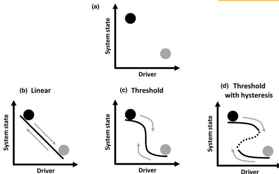
FIGURE 1 Trajectories for regime shifts in ecosystems. Ecosystems experience a regime shift when they show a large change in an ecosystem state (i.e. variables describing the ecosystem) (a). This change can be due to one or more environmental drivers and can be gradual or fast, leading to multiple relationships (unbroken black line) between ecosystem state and environmental drivers. The regime shift can be gradual if the ecosystem state changes linearly with the driver (b) or abruptly (c). In that case, the abrupt change associates with a threshold response to the environmental driver. In addition, the regime shift can show hysteresis if the direction of the change (grey arrow) is associated with different thresholds (d). In this case, bringing the driver back across the original threshold will not return the ecosystem to its previous state (broken black lines).
