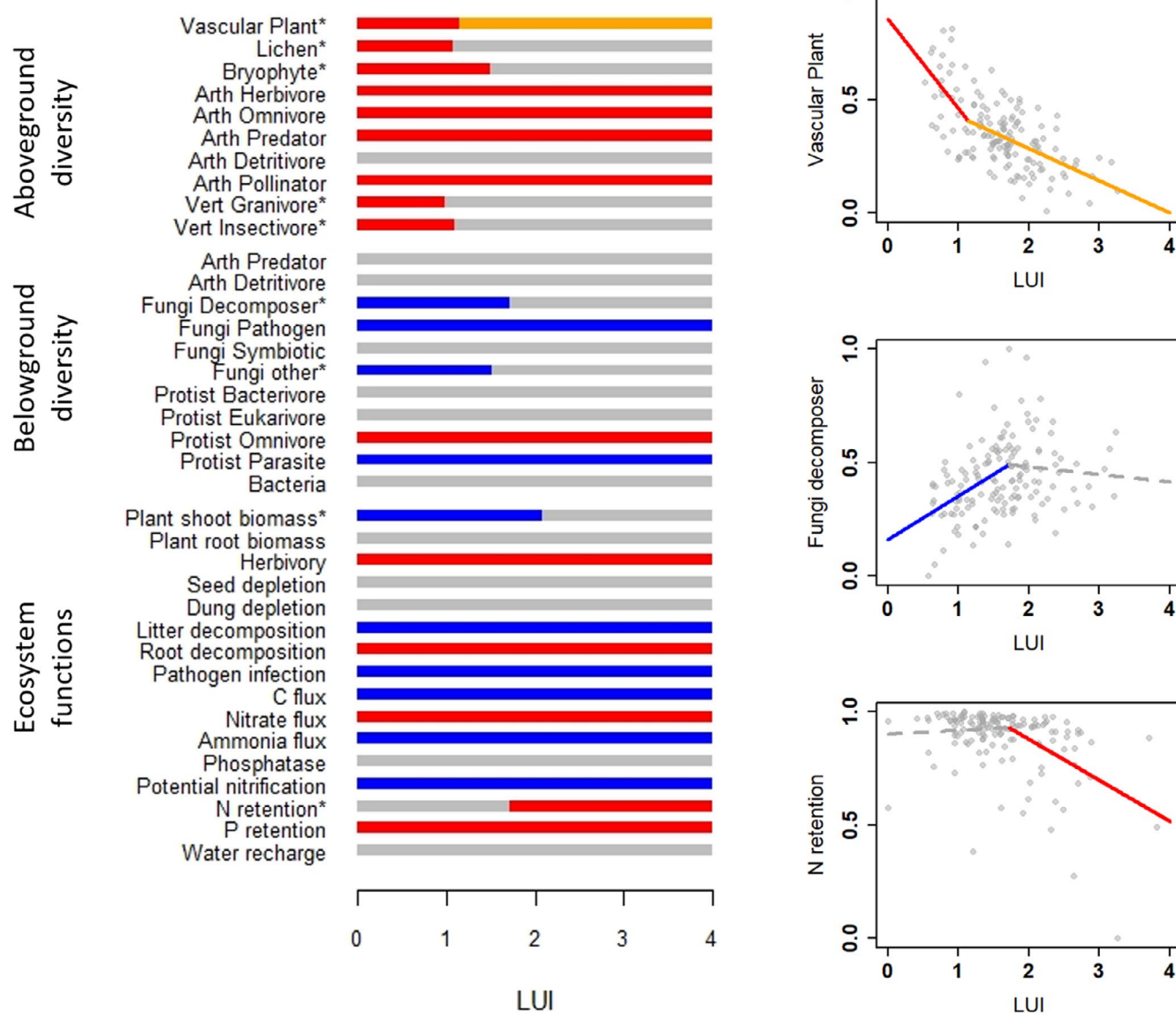
FIGURE 2 Threshold responses along LUI gradient for different taxa diversity and ecosystem functions. On the left, response to land use intensity (LUI) of all variables considered, including above- and below-ground diversity, and ecosystem functions. Different colours indicate different responses to LUI (red/orange = negative response; blue = positive response; grey = no response; vascular plant diversity always decreased with land use intensity but the strength of that decline was lower after the threshold, which is indicated as a shift from red to orange). *Indicates a variable showing a threshold response. On the right, one example of threshold response for above- (plants) and below-ground diversity (fungal decomposers) and ecosystem function (N retention).
