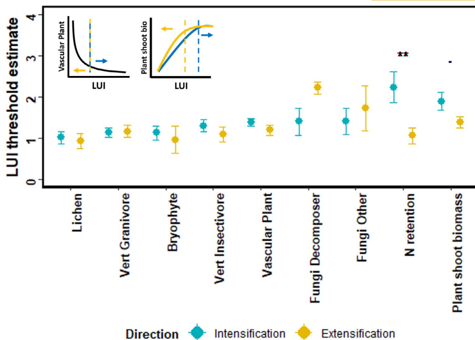
FIGURE 4 Variation in the Land Use Intensity (LUI) threshold depending on temporal changes in land use. Land use thresholds for each diversity and ecosystem function on plots where LUI had recently increased (intensification, blue line and dots) or decreased (extensification, orange line and dots). For diversity metrics, no threshold was affected by the direction of recent changes in LUI but ecosystem functions had different thresholds depending on whether LUI had recently increased or decreased, suggesting hysteresis and the presence of a critical transition between two ecosystem states. Inner subplots show (left) the threshold response of plant diversity to LUI, which is the same for plots where LUI had increased or decreased compared to the previous year; and (right) hysteresis for the threshold response of plant shoot biomass, where the threshold is different on plots where LUI had increased compared to the previous year (blue) or where it had decreased (yellow). ‘.’ p < 0.1 , ‘*’ p < 0.01 .
