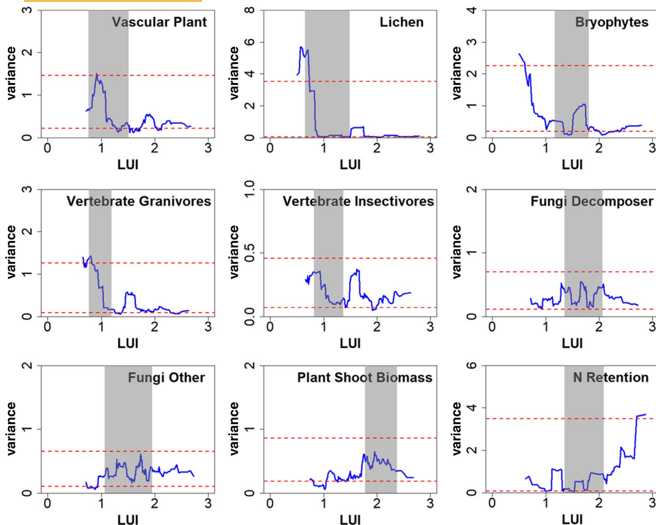
FIGURE 3 Variance for the considered taxa diversity and ecosystem functions showing a threshold response along the Land Use Intensity (LUI) gradient. The grey area represents the values along the gradient where a threshold was detected. Red dashed lines represent the confidence interval for the expected variance calculated based on bootstrapping the plots. Variance values higher than expected can be considered as indicative of a critical transition between ecosystem states.
