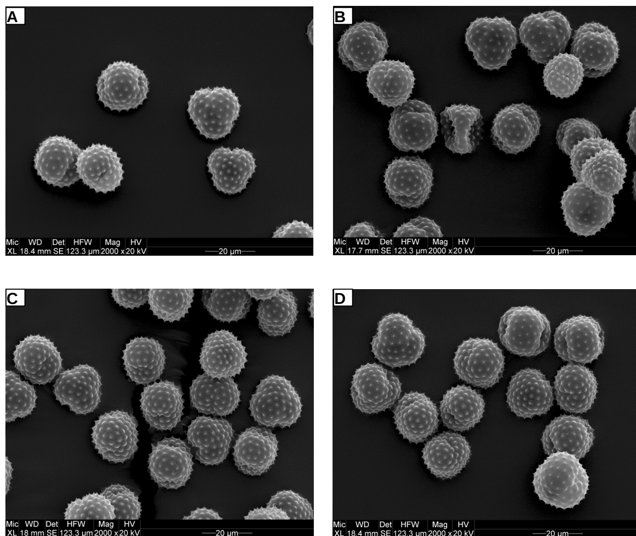
Figure 16: Scanning electron microscopy of ragweed pollen (A) Control. (B) Elevated CO 2 . (C) Drought. (D) Elevated CO 2 + drought. Bars 20 µm.
