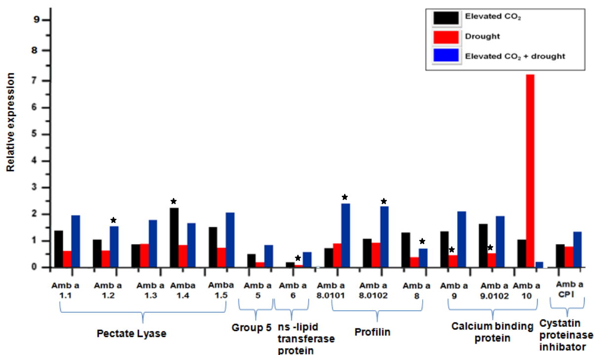
Figure 27: Real-time RT-PCR analysis for pollen allergen genes families, pectate lyase (Amb a 1.12 - 1.2 - 1.3 - 1.4 - 1.5), group 5 (Amb a 5), non specific lipid transferase protein (nsLTP) (Amb a 6), profilin (Amb a 8.0101-8.0102-8), calcium binding protein (Amb a 9-9.0102-10) and cystatin (Amb a CIP) was represented in second generation ragweed pollen (2011) treatments (elevated CO 2 , drought, elevated CO 2 plus drought). Transcript levels were normalised with respect to 16S-rRNA and \alpha -tubulin transcript levels. Mean values were obtained from three independent PCR amplifications. Pair-wise fixed reallocation randomisation test according to Pfaffl et al., (2002). * refers to significant difference between treatments ( P \leq 0.05 ) and control.
