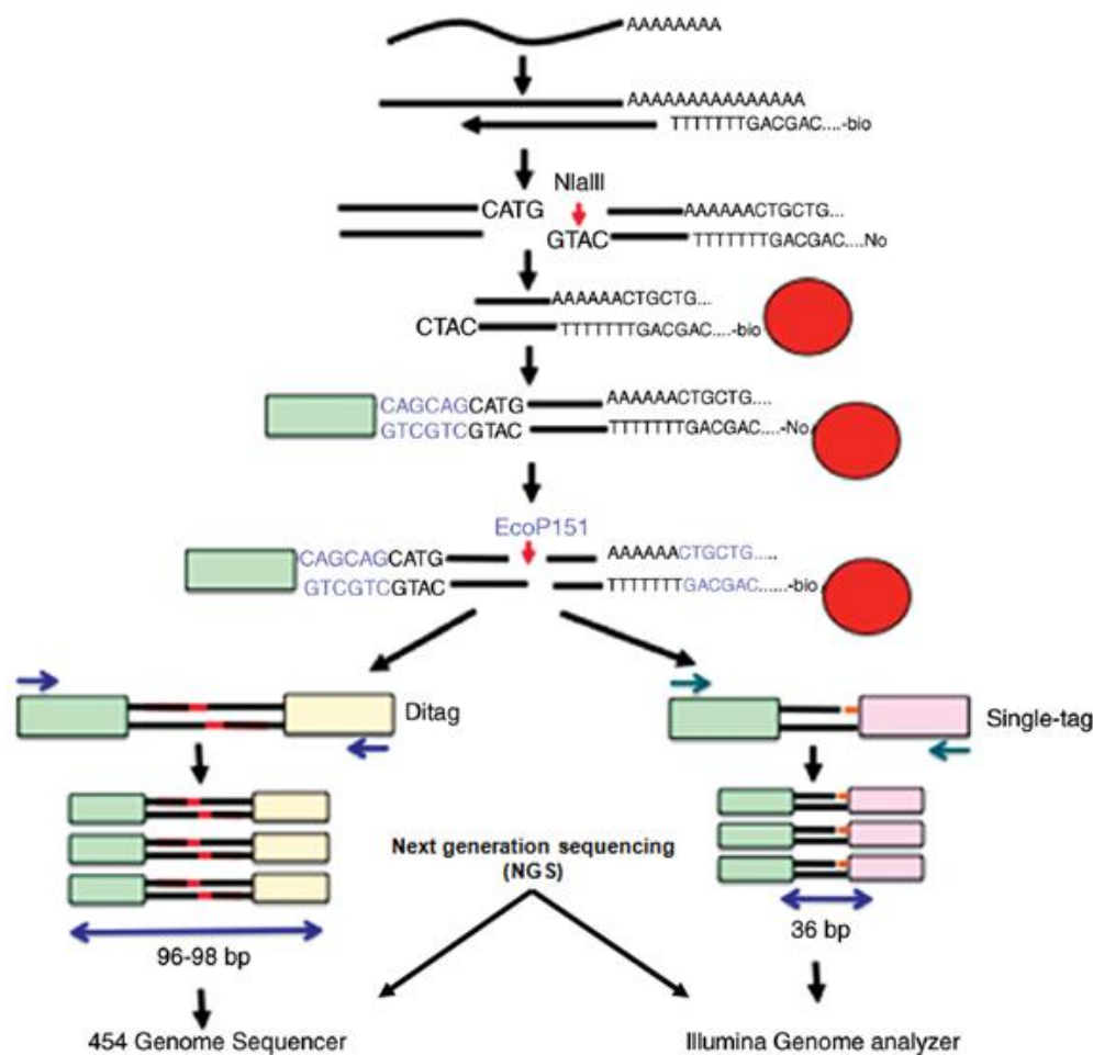
Figure 4: Schematic for DeepSuperSAGE. After EcoP15I digestion of linker (adapter)-ligated cDNA fragments immobilized on paramagnetic beads, ditags were formed for 454 pyrosequencing analysis (left) or another adapter was immediately ligated to the EcoP15I diges (Matsumura et al. 2012).
