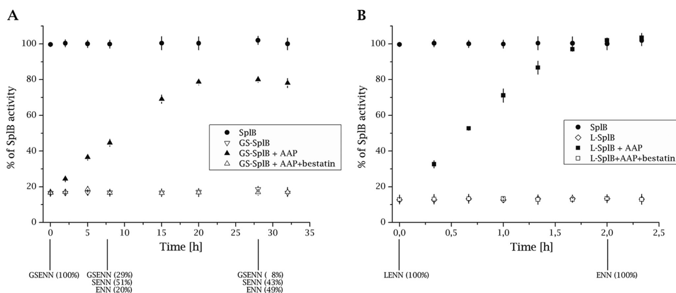
FIGURE 1. Removal of artificial N-terminal extension releases the proteolytic activity of GS-SplB and L-SplB. A, GS-SplB was incubated with AAP, and the proteolytic activity against Ac-WELQ-ACC (specific for SplB) was monitored. The activity is represented as a percentage of the maximum activity observed for the same concentration of SplB protease as the initial concentration of GS-SplB. Bestatin inhibits AAP activity. Samples were collected at indicated time points and subjected to N-terminal Edman degradation sequencing (results shown at the bottom of the panel). Activity of AAP remained unchanged during the experiment as monitored using Leu-pNa (not shown). B, same as in A but for L-SplB.
