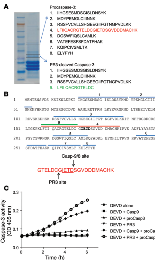
Figure 4. PR3 cleaves procaspase-3 at a site upstream of the canonical caspase-9 cutting site. (A) MS analysis of procaspase-3 and PR3-cleaved caspase-3. The expected position of procaspase-3 and the cleaved p20 fragment are indicated. The full-length procaspase-3 (top) and the 20-kDa fragment (bottom) were digested with endoproteinase Lys-C and analyzed by MS. (B) PR3 and caspase-9/8 cleaved procaspase-3 at different sites. Peptides in which one end followed the pattern of digestion by the endoproteinase Lys-C are underlined, and caspase-9/8 and PR3 cleavage sites are indicated. (C) Cleavage of procaspase-3 led to caspase-3 activation. PR3 was not able to cleave the DEVD substrate by itself. Results are representative of 3 independent experiments.
