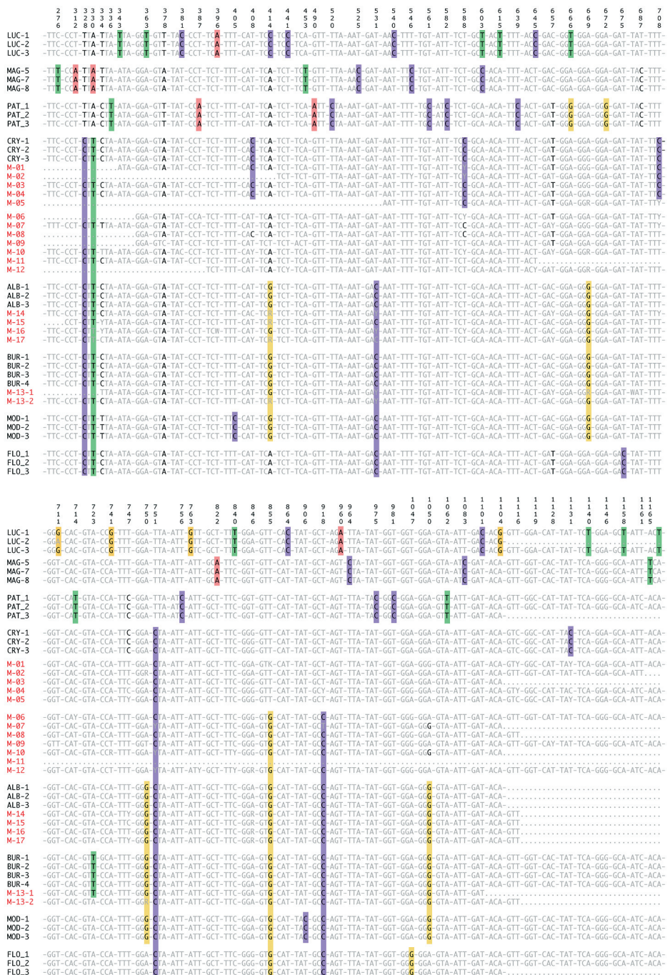
Fig. 3: Alignment of all parsimonious informative triplets (with uninformative sites deleted -), and with a pointer for position number (numbered for total COI) and codon position. Diagnostic (= private) positions marked with colour green = Thymine, violet = Cytosine, red = Adenine and yellow = Guanine.
