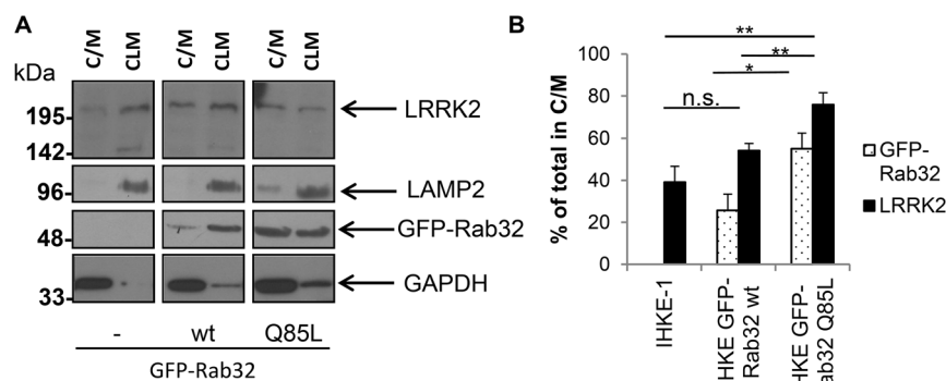
Figure 6. Subcellular fractionation analysis of endogenous LRRK2 in IHKE-1 cells overexpressing GFP-Rab32 wt or GFP-Rab32 Q85L. (A) IHKE-1 cells either untransfected (–) or stably overexpressing GFP-Rab32 wt or GFP-Rab32 Q85L were mechanically disrupted and fractionated by differential centrifugation. Fractions received either contained lysosomes and mitochondria (CLM) or cytosol and light membranes (C/M). Western blot analysis to detect the lysosomal marker LAMP2, GAPDH, Rab32 and LRRK2 were performed with the fractions derived from the different IHKE-1 cells. (B) Quantification of Western blot signal intensities using the gel analyzer functionality of ImageJ. The signal intensity for both the C/M and the CLM fraction was added and set to 100%. The graph shows the % of GFP-Rab32 and endogenous LRRK2 in the C/M fraction of the different cell lines. n = 6 independent experiments. Error bars represent S.E.M.; n.s. = not significant; * = p < 0.05 ; ** = p < 0.01 . doi:10.1371/journal.pone.0111632.g006
