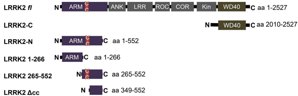
Figure 1. LRRK2 constructs used in this study. ARM: armadillo repeats; ANK: ankyrin repeats; LRR: leucine rich repeats; ROC: Ras of complex; COR: C-terminal of ROC; Kin: kinase domain; WD40: WD40 domain; c/c: coiled coil motif (aa 319–348). doi:10.1371/journal.pone.0111632.g001
