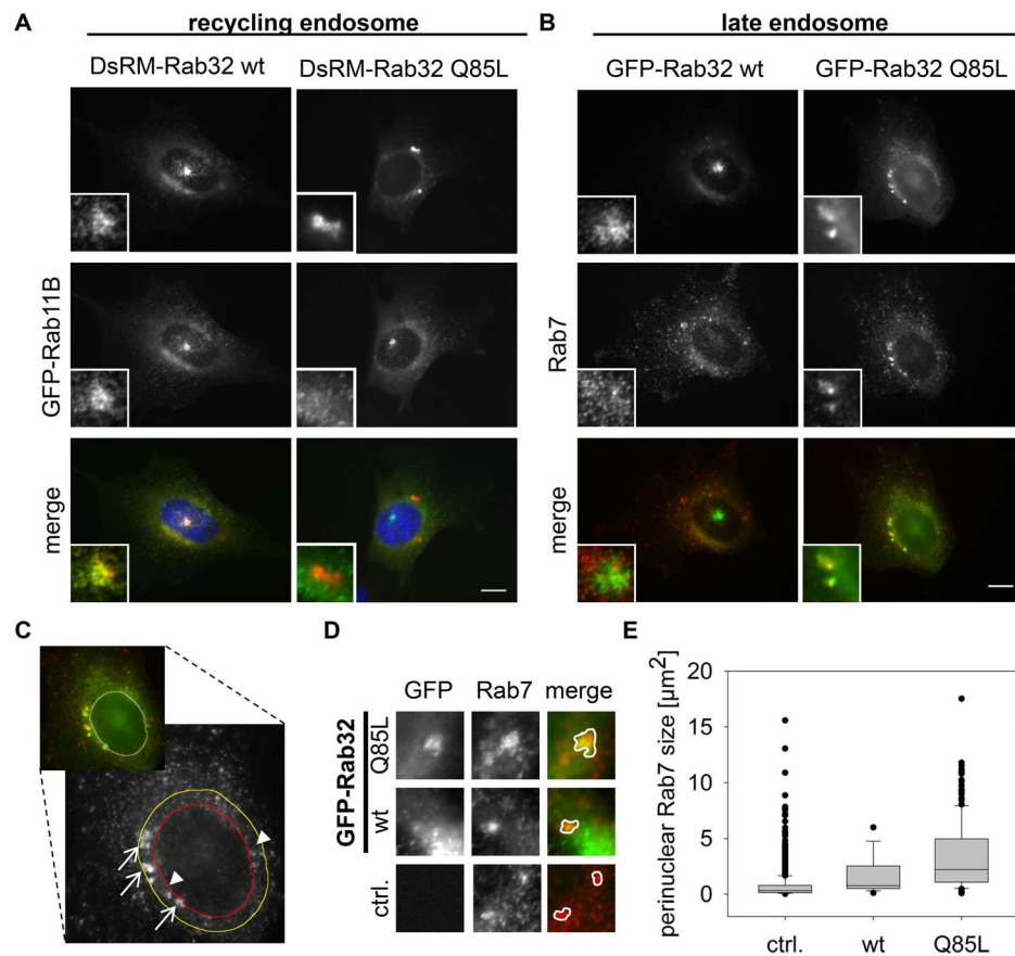
Figure 4. Co-localization analysis of Rab32 wt and the constitutively active mutant Rab32 Q85L with different endosomal markers. (A) NIH3T3 cells were co-transfected with plasmids encoding the recycling endosome marker GFP-Rab11B and DsRed-Monomer-Rab32 wt or DsRed-Monomer-Rab32 Q85L, fixed and analyzed by fluorescence microscopy. Scale bar = 10 \mu\text{m} . (B) Cells were transfected with plasmids encoding for GFP-Rab32 wt or GFP-Rab32 Q85L followed by fixation and subsequent immunofluorescence staining of Rab7. Scale bar = 10 \mu\text{m} . (C–E) NIH3T3 cells expressing either GFP-Rab32 wt or GFP-Rab32 Q85L were fixed and stained for Rab7. (C) Microscopic analysis of GFP-Rab32 Q85L that co-localized with endogenous Rab7 (arrows) in the perinuclear area. Non co-localizing Rab7 was indicated by arrowheads. The perinuclear area was defined by the red (outlines nucleus) and the yellow line (outer border for perinuclear area). The image illustrates the cellular area used for the following analysis. (D) Rab7 perinuclear aggregates co-localizing with GFP-Rab32 wt or GFP-Rab32 Q85L and non co-localizing ones. ctrl. = control (untransfected IHKE-1 cells) (E) Quantification of perinuclear Rab7-positive structures. ctrl. (control): perinuclear Rab7 in untransfected cells; wt/Q85L: perinuclear Rab7 co-localizing with GFP-Rab32 constructs. control/Rab32 wt/Rab32 Q85L: n = 1660/18/167 structures in 67/18/60 cells, 1/1/3 independent experiments. Statistical significance was tested by a Student's T-test: p_{\text{control-wt}} = 0.02 ; p_{\text{control-Q85L}} < 0.005 ; p_{\text{wt-Q85L}} = 0.02 . Scale bar = 10 \mu\text{m} . doi:10.1371/journal.pone.0111632.g004
