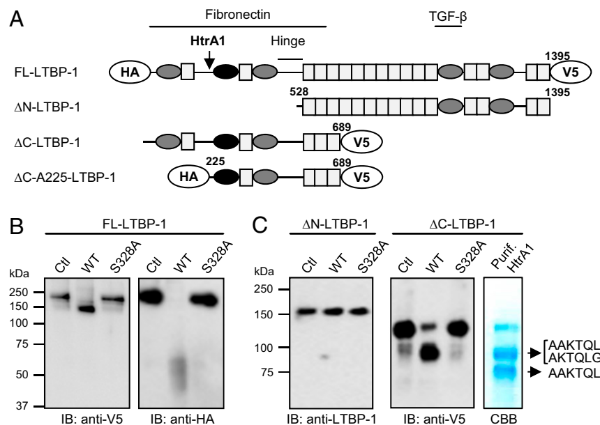
Fig. 4. Mapping of the HtrA1 cleavage site within LTBP-1. (A) Domain organization of LTBP-1 including cysteine-rich domains (gray ovals), a hybrid domain (black oval) and EGF-like domains (rectangles). The protease-sensitive hinge region as well as binding regions for fibronectin and TGF-β are shown. The HtrA1 cleavage site is indicated by an arrow. Numbers represent amino acids. The various LTBP-1 constructs used in this study are depicted. HA: Hemagglutinin tag; V5: V5 tag. (B) Medium from HEK293 cells expressing full-length (FL-) LTBP-1 was exposed to medium from vector- (Ctl), HtrA1 WT-, or HtrA1 S328A-transfected cells and LTBP-1 analyzed by immunoblotting. (C) HEK293 cell-derived ΔN-LTBP-1 (Left) or ΔC-LTBP-1 (Center) was treated with control, HtrA1 WT-, or HtrA1 S328A-containing medium and immunoblotting was performed. Purified ΔC-LTBP-1 (Right) was treated with purified HtrA1 and upon SDS/PAGE and Coomassie brilliant blue (CBB) staining two proteolytic fragments were isolated and subjected to Edman degradation. The resulting amino-terminal sequences are indicated. Note that the smaller fragment (~75 kDa) could not be detected by an anti-V5 antibody indicating carboxyl-terminal processing.
