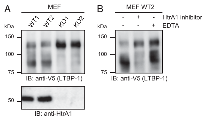
Fig. 5. LTBP-1 processing by endogenous HtrA1. (A) Concentrated culture medium from wild-type (WT) or HTRA1 knockout (KO) MEF lines was incubated with ΔC-LTBP-1-containing medium. LTBP-1 and HtrA1 were analyzed by immunoblotting using anti-V5 and anti-HtrA1 (16C8) antibodies. (B) ΔC-LTBP-1 was exposed to medium from the HtrA1-WT2 line in the absence or presence of a selective HtrA1 inhibitor or EDTA, before LTBP-1 was immunodetected.
