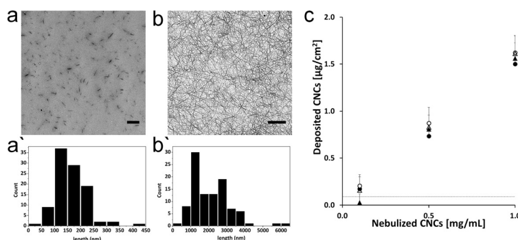
Figure 2 Morphology and quantification of deposited CNC aerosols. Transmission electron microscopy images of 1 mL nebulised c-CNCs (a) and t-CNCs (both 0.5 mg/mL) (b) deposited on pre-coated, protein rich copper grids using the ALICE system resulting in a deposited dose of 0.81 \pm 0.03 \mu\text{g}/\text{cm}^2 . Histograms show the size distribution as counts (y-axis) and length (nm) (x-axis) of c-CNCs (a') and t-CNCs (b'). Dimensions are measured from pictures derived from nebulisations leading to mostly individually deposited fibers (c-CNCs 0.5 and 0.1 mg/mL; t-CNCs 0.1 mg/mL). Average dimensions were calculated from 100 individual measurements of 3 individual nebulisations (n = 3). Quantification of deposited c-CNCs and t-CNCs after nebulisation at 0.1, 0.5 and 1 mg/mL was performed using two independent methods (n = 3) (c). Dots (o) represent results for c-CNCs, triangles (Δ) t-CNCs; filled symbols = QCM data, empty symbols = Anthrone data. The dotted line (...) displays the detection limit of the QCM (90 ng/cm²). Scale bars represent 1 μm.
