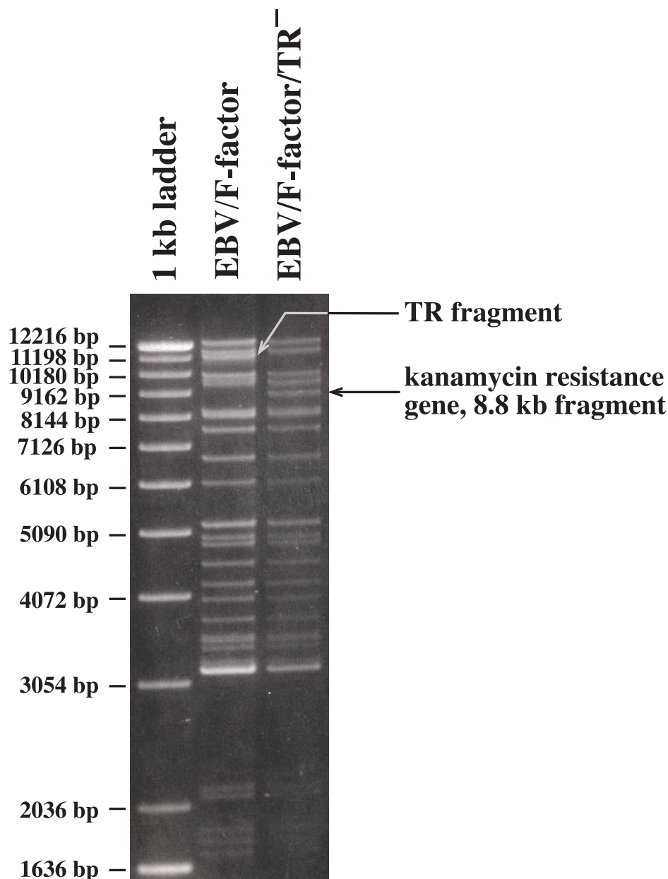
FIG. 2. Restriction fragment analysis of TR - mutant DNA in comparison with the wild-type B95.8/F factor DNA. DNA was purified from a chloramphenicol- and kanamycin-resistant E. coli clone and digested with the Bam HI restriction enzyme. The restriction pattern of the modified B95.8/F factor DNA was compared with the one obtained with wild-type B95.8/F factor DNA. Both restriction fragment patterns were identical with one exception. A new fragment was generated by the exchange of the Bam HI fragment that carries the TRs (disappearance of the 11.2-kb fragment in EBV/F factor) against the kanamycin-resistance gene (appearance of an 8.8-kb fragment in EBV/F factor/TR - DNA).
