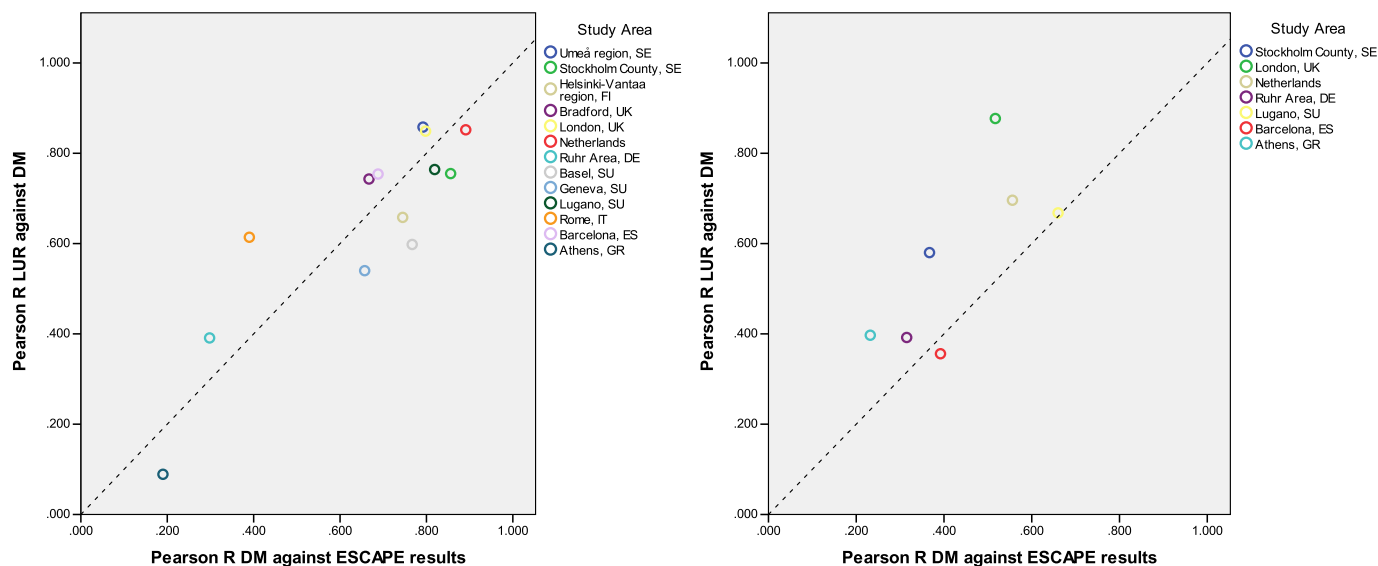
Fig. 3. Scatterplots of Pearson R 's between the LUR–DM and DM–ESCAPE comparisons for both \text{NO}_2 and \text{PM}_{10} .
