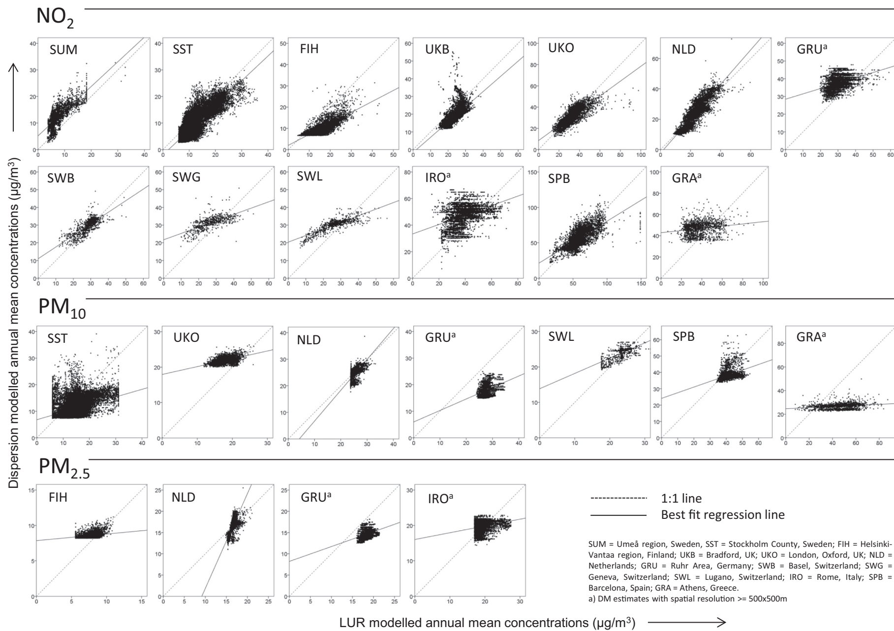
Fig. 1. Scatter plots of DM (y-axis) against LUR (x-axis) estimates (µg/m 3 ) at residential addresses for NO 2 , PM 10 and PM 2.5 .
