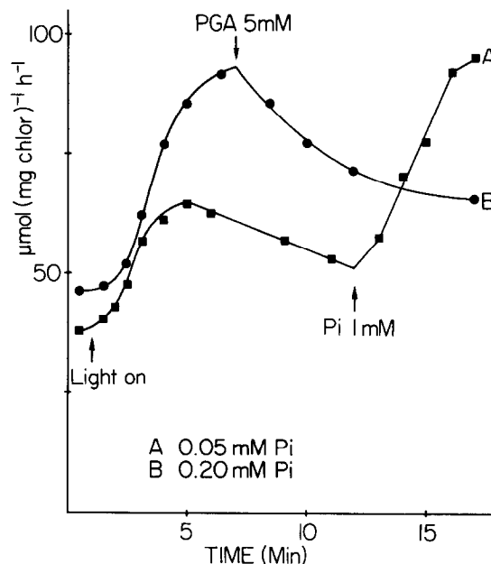
Fig.2. RuBP carboxylase in chloroplasts. P_i dependency of the light activation. Expt. A: 0.05 mg chl/ml; Expt. B: 0.1 mg chl/ml; P_i in medium and further additions are indicated in the figure. expt. 303 and 308.
