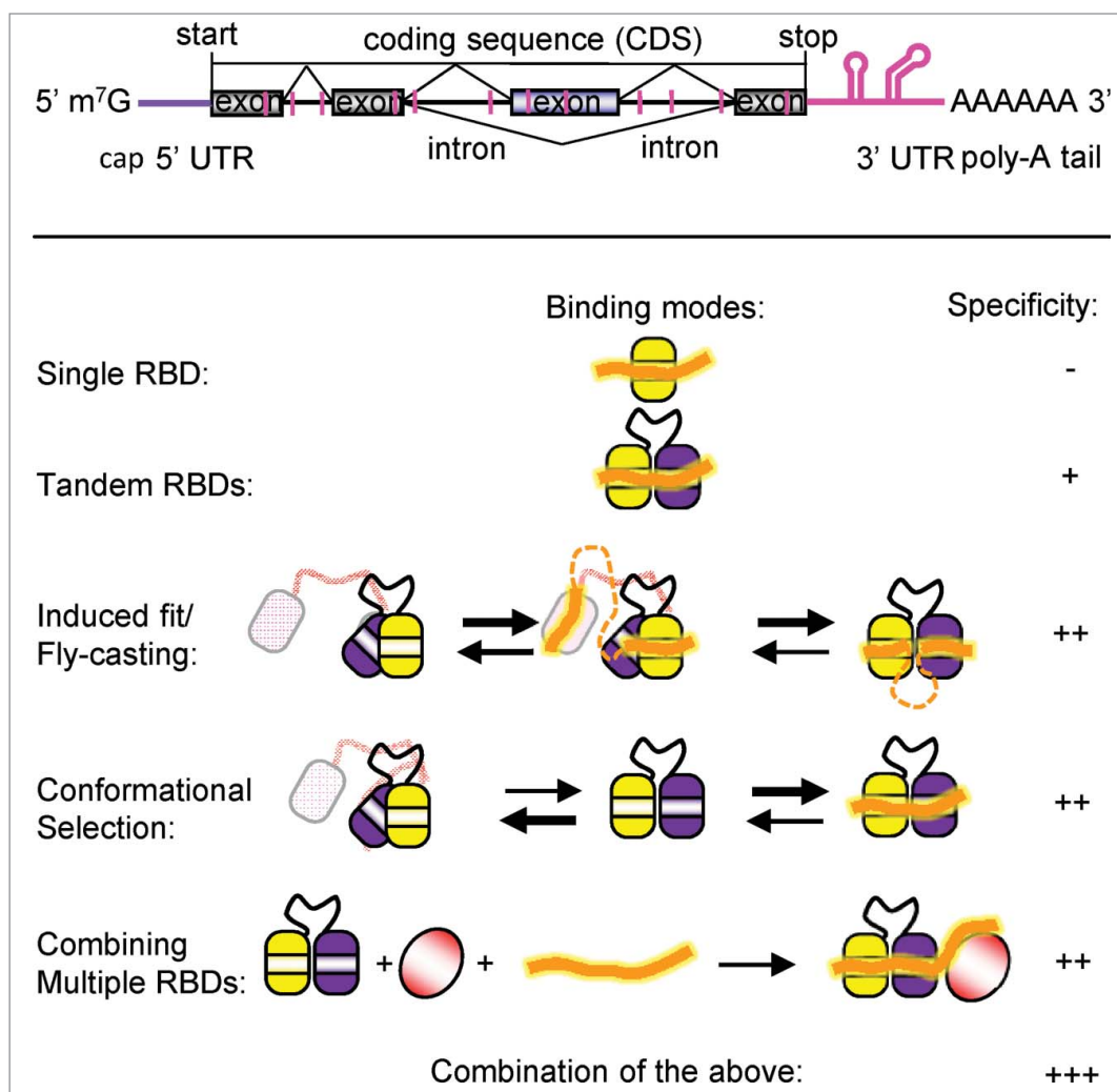
Figure 1. Recognition of mRNA by RNA binding proteins (RBPs). Top: A schematic view of a pre-mRNA indicating introns, exons, the poly(A)-tail, the untranslated regions (UTRs), and cis elements (pink). Bottom: Different binding modes how regulatory RBPs can bind to poly(U) cis elements. A combination of these modes yields the highest binding specificity.
