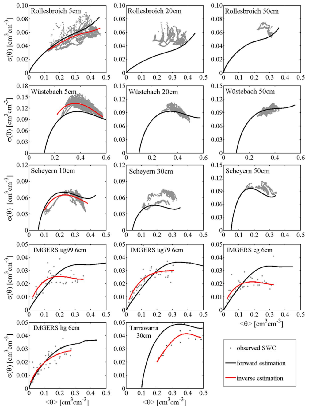
Figure 2. Field-observed \sigma_{\theta}(\langle\theta\rangle) data from the three TERENO test sites (Rollesbroich, Wüstebach, and Scheyern), the four IMGERS experiment sites (ug99, ug79, cg, and hg), and the Tarrawarra test site as well as the forward and inverse estimation results.
