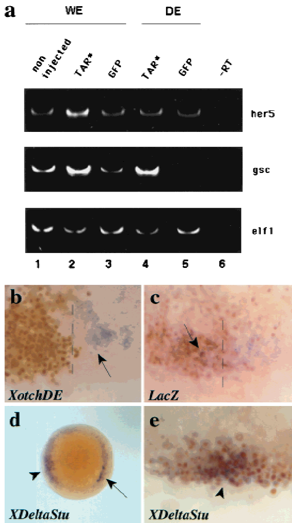
Figure 8. her5 expression requires positive cell interactions and an inhibition of Notch/Delta signaling. (a) The induction of her5 by Tar* requires positive cell interactions. RNA was extracted from whole embryos (WE, 1–3) or dissociated embryos (DE, 4–5) injected with 1 pg of Tar* RNA (2,4) or 100 pg of GFP RNA (3,5), and subsequently processed for RT-PCR. Elf1 serves as a loading control. Lanes 1 and 6 are samples from noninjected embryos treated with or without reverse transcriptase. (Endodermal) Expression of her5 is not induced upon Tar* injection when the cells of the injected embryos are dissociated; in contrast, gsc induction by Tar* is cell autonomous (cf. lanes 2 and 4 in each case). The basal level of her5 expression, maintained in dissociated cells (lane 5), probably corresponds to remnants of the early ubiquitous (nonendodermal) phase of her5 expression (see text). (b–e) Embryos were injected at the 16-cell stage into a marginal blastomere with 2 pg of capped XotchDE + 3 pg of lacZ RNAs (b), 3 pg of lacZ RNA (c), or 2 pg of XDelta Stu + 3 pg of lacZ RNAs (d,e), and tested for her5 (in situ hybridization, blue) and betagalactosidase (immunocytochemistry, brown nuclei) (except in d) expressions at the shield stage. (a–c, e) Flat-mounts of the injected areas; (d) animal pole view of the embryo shown in e, photographed prior to betagalactosidase detection. The injected areas in b,c overlapped with the endogenous axis (dorsal midline indicated by the broken line), whereas they are ventrally located in d,e. Endogenous her5 expression (arrows in b–d) is inhibited by XotchDE (cf. b with c where no inhibition is observed following expression of lacZ alone). In contrast, following XDelta Stu misexpression, her5 induction (arrowheads in d,e) occurs in deep cells of the margin (d), which derive from the injected blastomere (cf. blue and brown in e).
